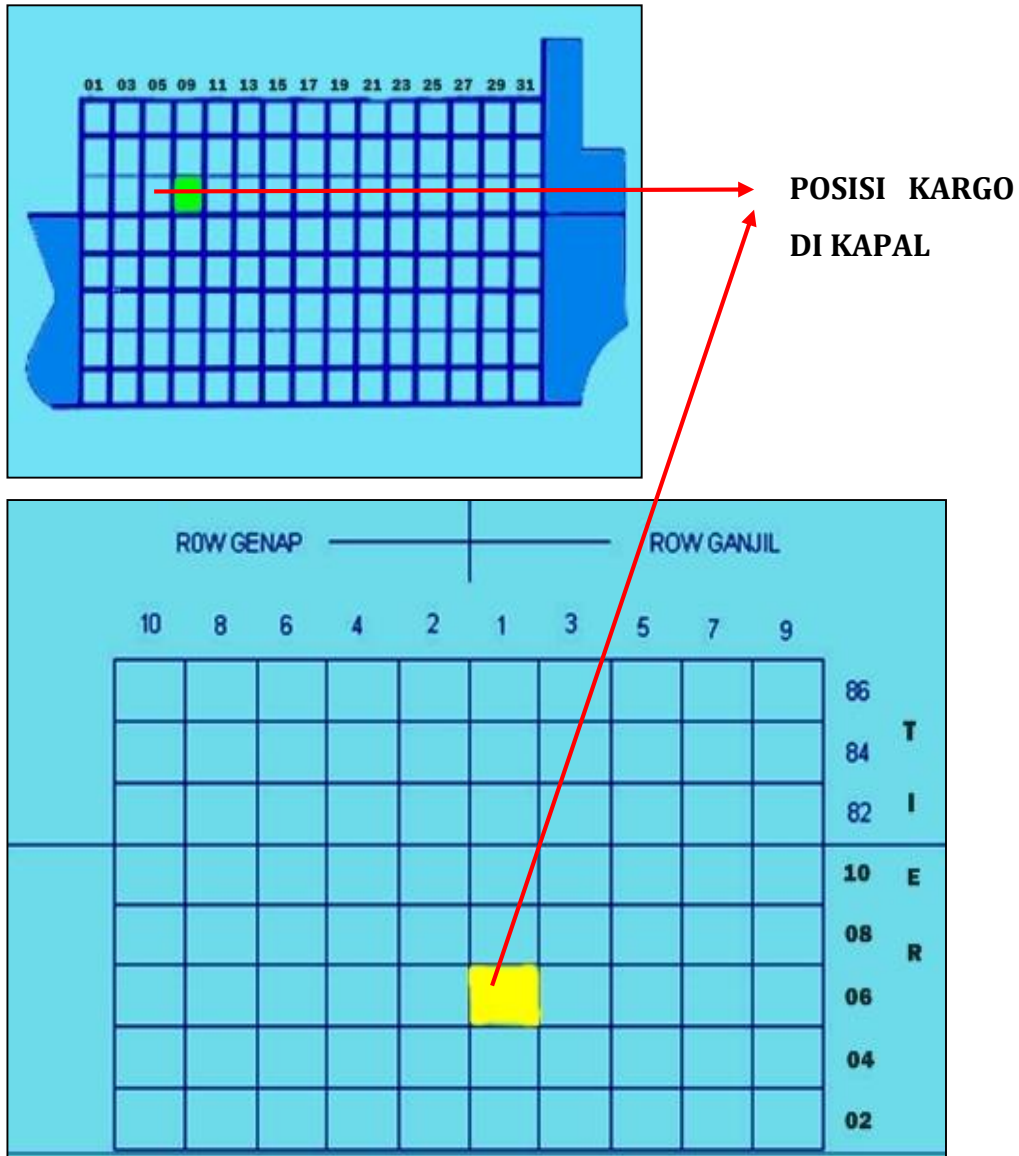
Gambar 33. General Bay Plan Kapal Container
