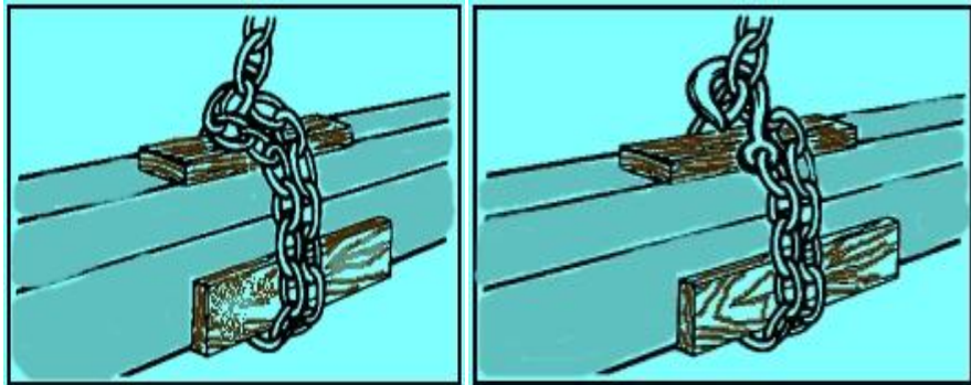
Gambar 10. Sling Rantai ( Chain Slings )
