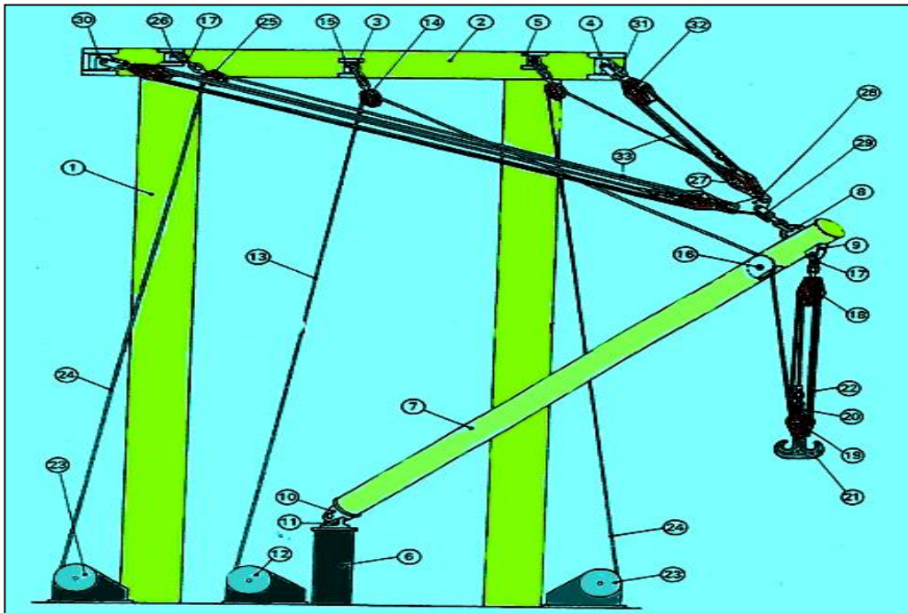
Gambar 5. Twin span tackle derrick rig for heavy loads
