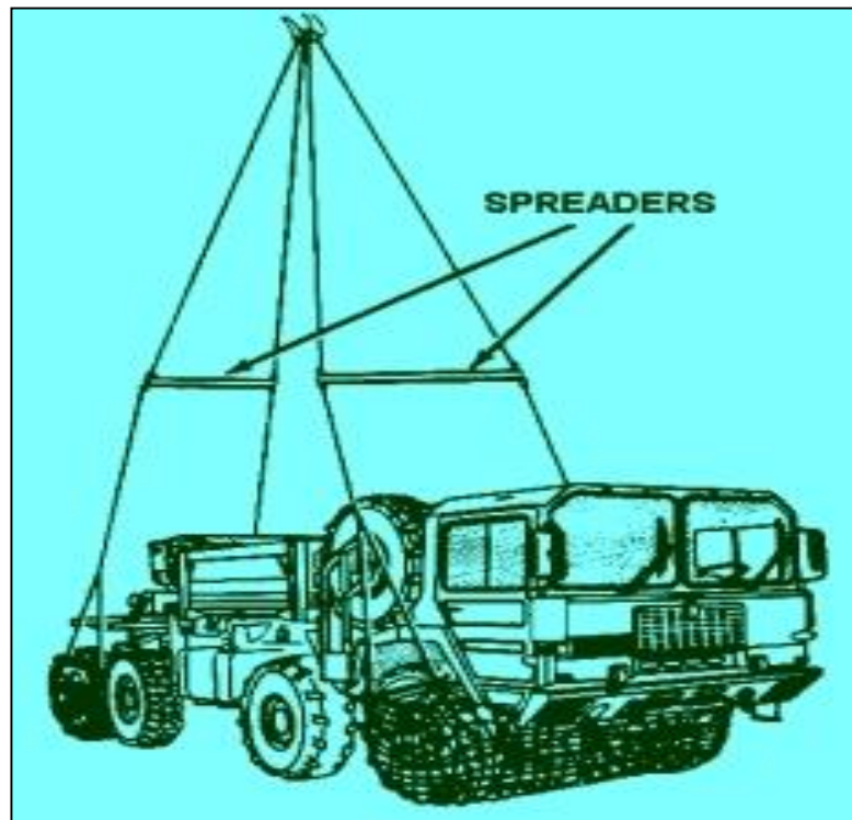
Gambar 17. vehicle spreader with wheel nets
