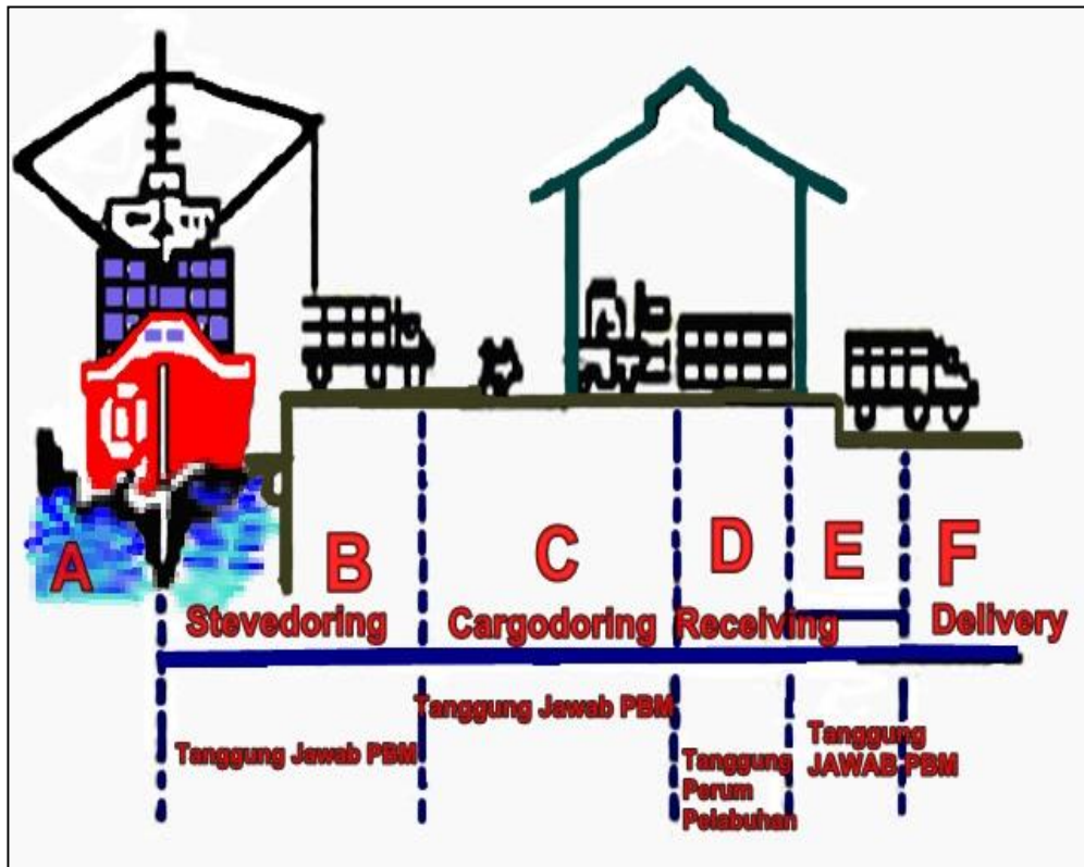
Gambar 25. Terminal Operator
