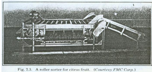
Fig. 7.3. A roller sorter for citrus fruit. (Courtesy FMC Corp.)
