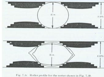
Fig. 7.3c. Roller profile for the sorter shown in Fig. 7.3b.
